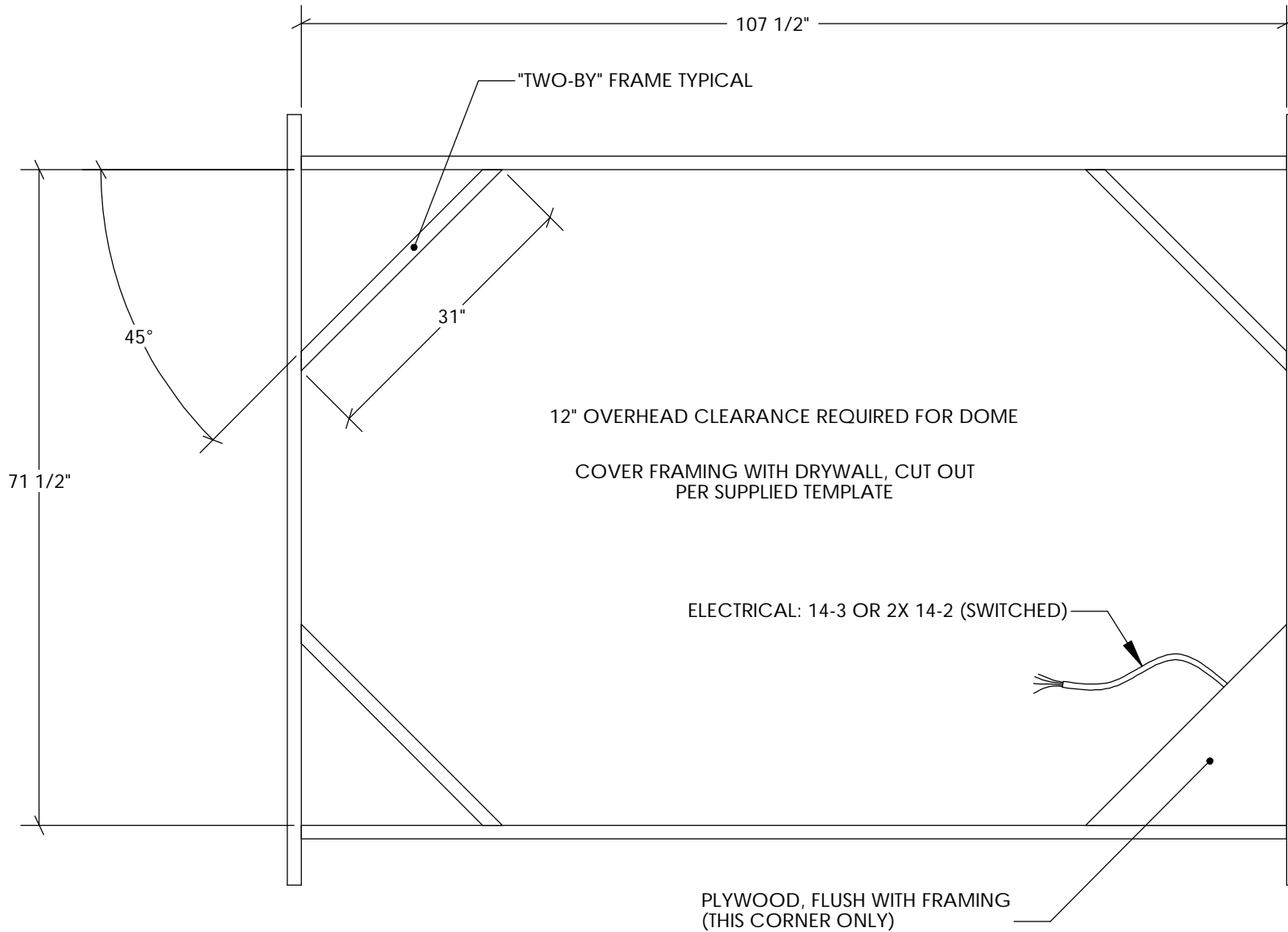
VIEW LOOKING UP TO CEILING
